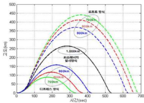
Altitude Characteristics
