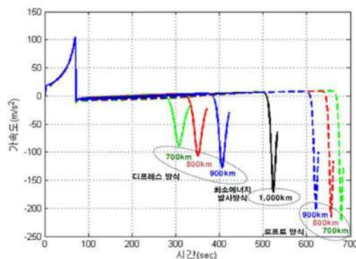
Acceleration Characteristics
