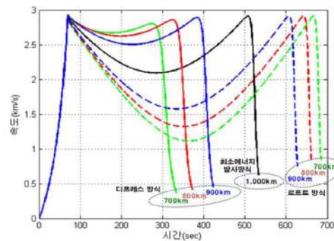
Speed Characteristics
